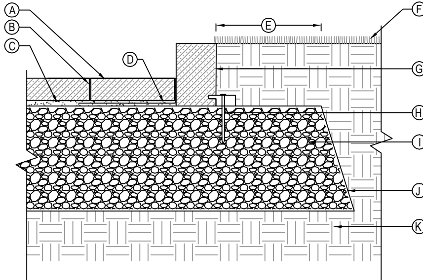
SECTION
